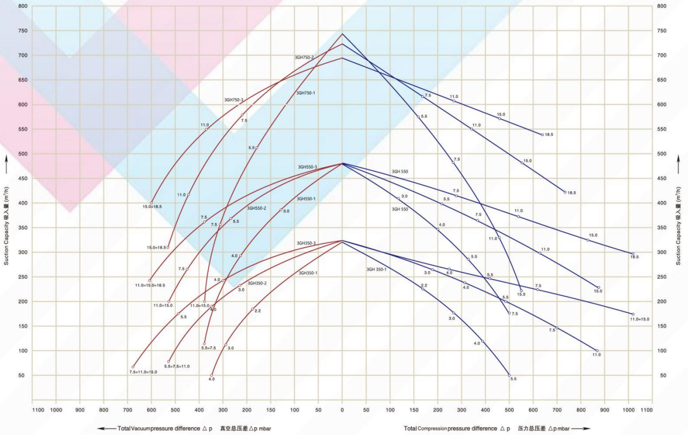
Vacuum Compression Selection Diagram 真空压缩图表 60Hz
